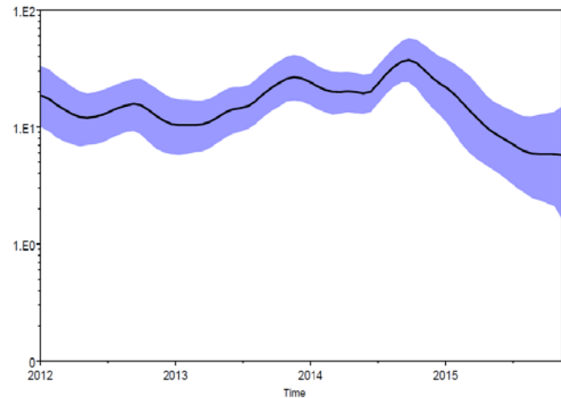
Fig. 3. Genetic diversity plot, Pakistan, 2012–2015
